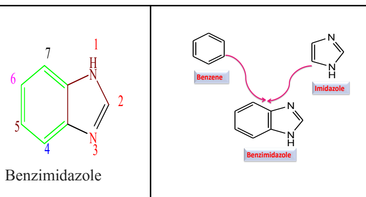
Fig. 4 The basic structure of benzimidazole
